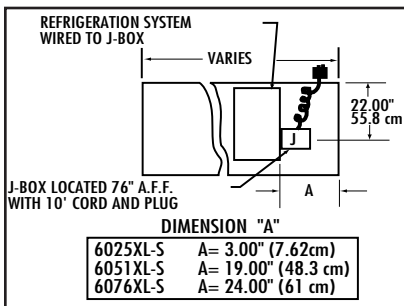
Mechanical Detail
